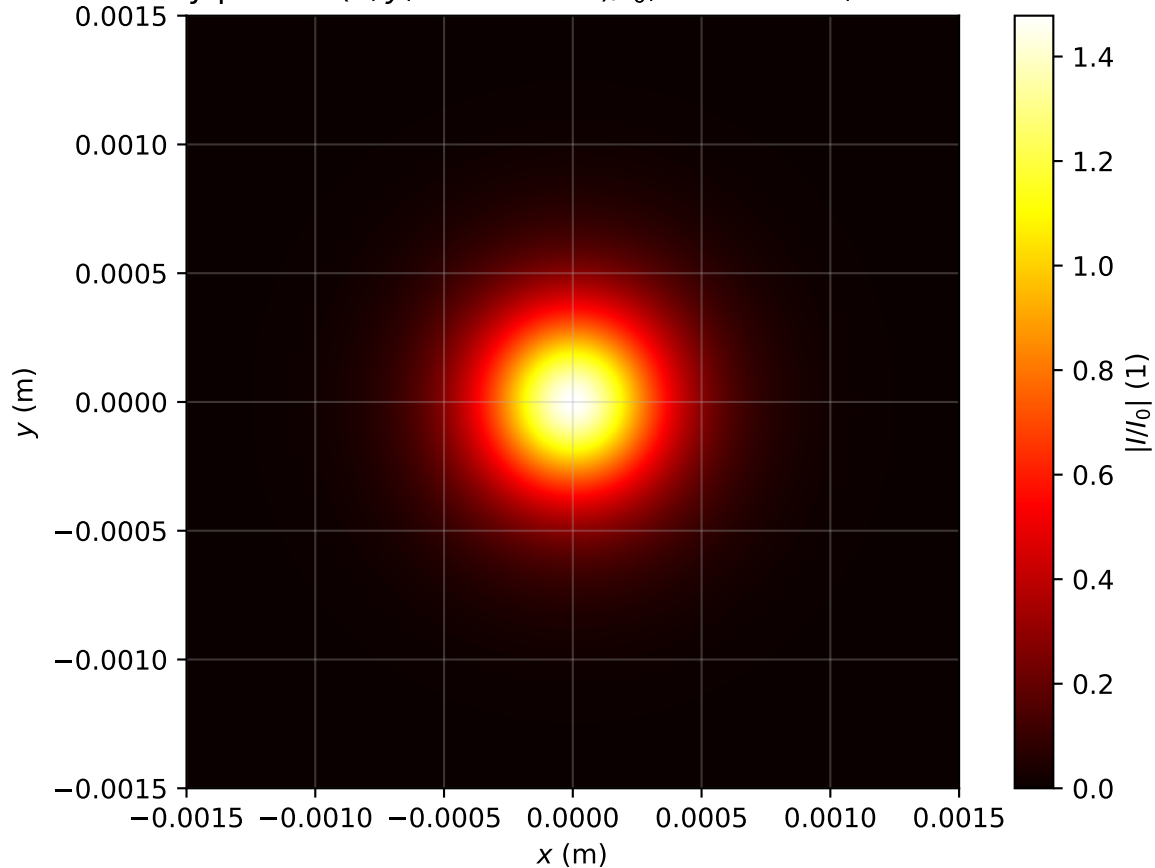
Intensity profile I(x, y, z = 3.582m)/I_0 , Pin=0.9Pcr, artificial time
